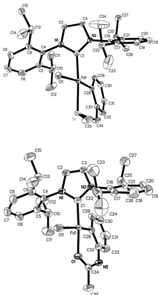
Figure 1. ORTEP representation of the single-crystal X-ray structures of complexes 9 (upper) and 11 (lower). The thermal ellipsoids were drawn at the 30 % probability level and the hydrogen atoms and co-crystallising solvent molecules (for complex 11 ) have been omitted for clarity.
