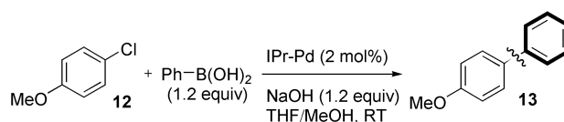
Scheme 2. Cross-coupling reaction of a deactivated substrate, p -chloroanisole ( 12 ), and pre-activated phenylboronic acid under non-basic conditions at room temperature mediated by the IPr-Pd precatalyst with various disposable ligands.
