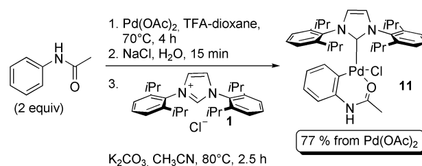
Scheme 4. Preparative synthesis of 11 on a 1.5 g scale.
