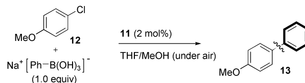
Scheme 3. Cross-coupling reaction of a deactivated substrate, p -chloroanisole ( 12 ), and sodium phenyltrihydroxyborate mediated by complex 11 in air.
