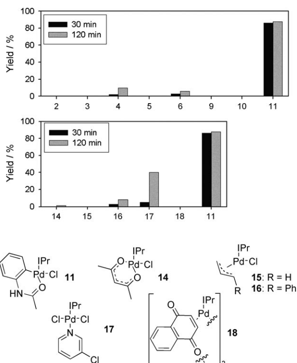
Figure 2. Evaluation of the catalytic activity of the NHC-palladacycle library (upper panel) and comparison of the catalytic activity of IPr-cyclopalladated acetanilide complex 11 with popular, commercially available IPr-Pd precatalysts (lower panel) in the model reaction (Scheme 2).
