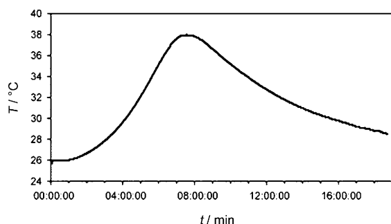
Figure 3. Thermal profile of the reaction of p -chloroanisole ( 12 ) and sodium phenyltrihiydroxyborate in air mediated by complex 11 (Scheme 3).
