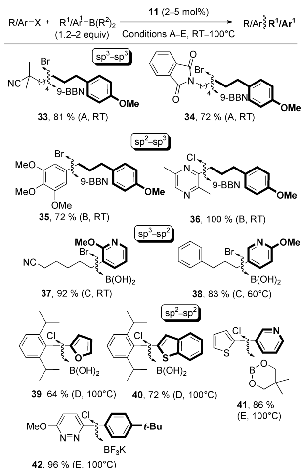
Scheme 6. Cross-coupling reactions of aryl and alkyl chlorides and bromides with alkyl bromides and arylboronic acids, esters and potassium trifluoroborates in various possible combinations mediated by 11 . The yields are of isolated chromatographically homogeneous materials (average from two runs), non-optimised for time and catalyst loading. Conditions: A) 4 mol % 11 , K 3 PO 4 /H 2 O, dioxane; B) 4 mol % 11 , K 3 PO 4 , THF/H 2 O; C) 4 mol % 11 , t BuOK, dioxane/MeOH; D) 5 mol % 11 , K 3 PO 4 , dioxane/H 2 O; E) 2 mol % 11 , K 3 PO 4 , dioxane/H 2 O.
