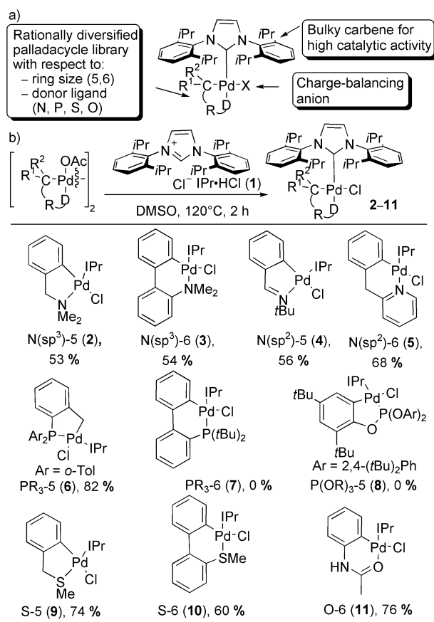
Scheme 1. Rationally diverse library of NHC-palladacycles (a) prepared by a novel, atom-economic method (b).
